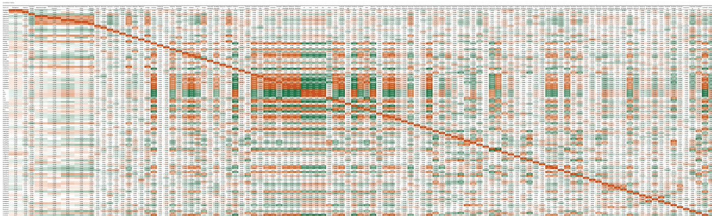
Supplementary Figure 1. The correlation matrix derived from the least absolute shrinkage and selection operator.
