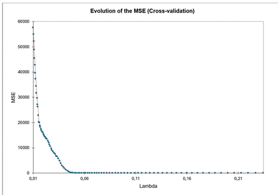
Supplementary Figure 2. Correlation of mean standard error (MSE) with lambda parameter.
