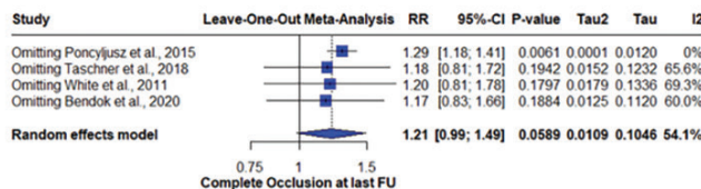
Supplementary Figure 1. Leave-one-out sensitivity analyses evaluating the robustness of pooled estimates across key outcomes. Each panel illustrates the impact of sequentially omitting individual studies on the pooled effect size under a random-effects model. (a) Immediate complete occlusion, (b) packing density, (c) complete occlusion at last follow-up. RR, risk ratio; CI, confidence interval.
